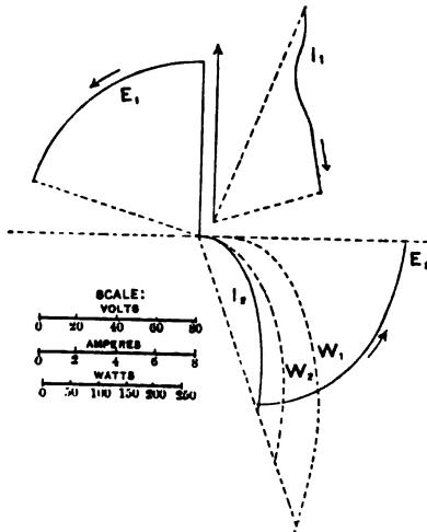
FIG. 19.—Constant Potential, Step Up, Arm at 150^\circ .
